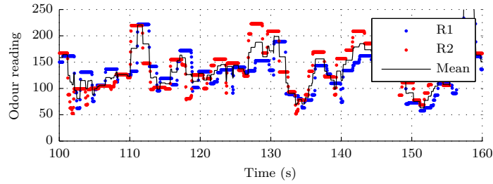
Figure 18.7 – Max-filtered odour measurements for robots A/R1 (left, front) and B/R2 (left, back), and resulting mean c_l .
