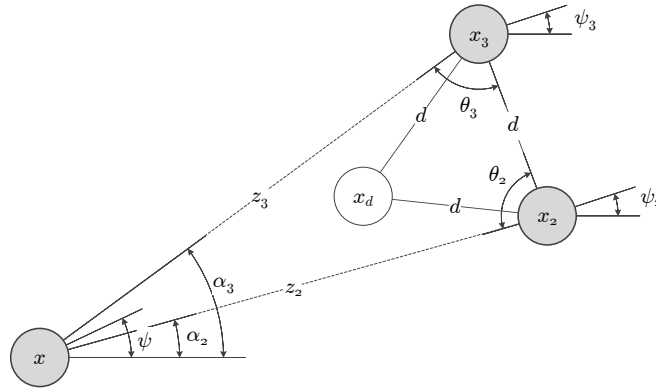
Figure 11.1 – System of three vehicles (1, 2, 3) and their intended triangular formation ( x_d, x_2, x_3 ). Vehicle 1 is the follower, and vehicles 2 and 3 are the leaders. The image shows many of the relevant parameters, including the formation and independent vehicle headings, as well as the relationships (ranges and bearings) between them.
