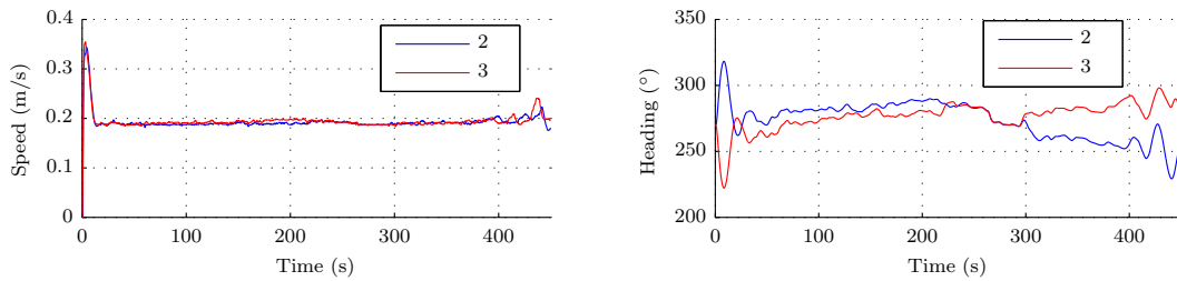
Figure 25.5 – Actual speed and heading of the leaders for the experiment in Figure 25.3a. The up-flow direction is 270°.
