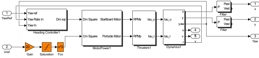
Figure 7.1 – Top-level view of the MEDUSA Simulink model.
