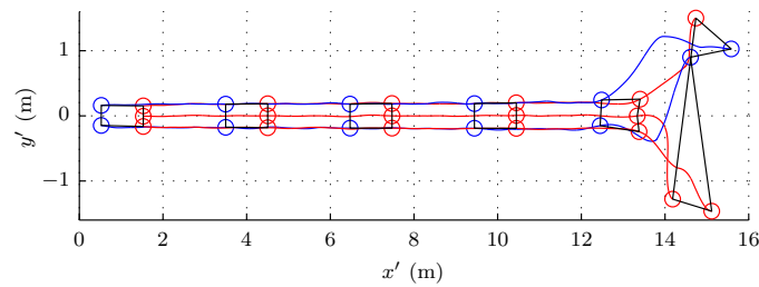
Figure 18.8 – Robot trajectories for a rectangular formation in a plume with growth rate \gamma = 4 \times 10^{-7} \text{ m}^2 \text{ s}^{-1} . The trajectories of the front robots are traced in blue and those of the back robots are traced in red. Black lines connect the robot positions at intervals of approximately 35 s.
