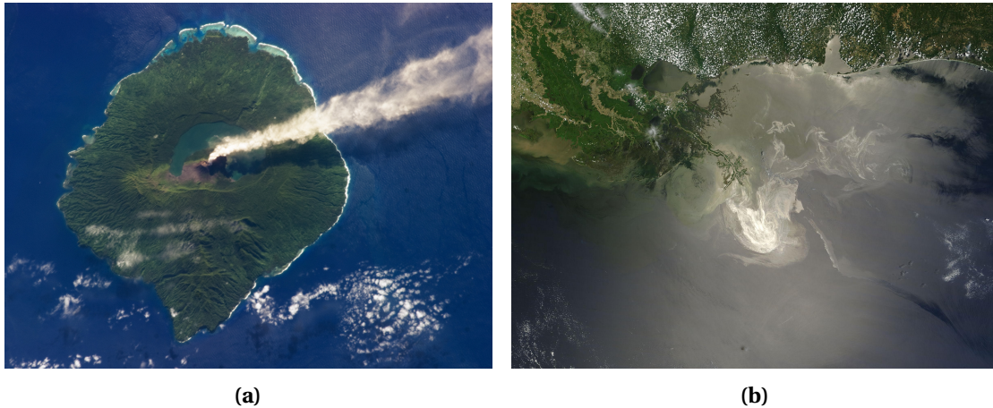
Figure 1.1 – Examples of plumes in the air and water. (a) Volcanic plume emanating from the Gaua Island eruption, Vanuatu, May 2013. (b) Oil plume resulting from the Deepwater Horizon spill, Gulf of Mexico, May 2010. (Image credit: NASA)
